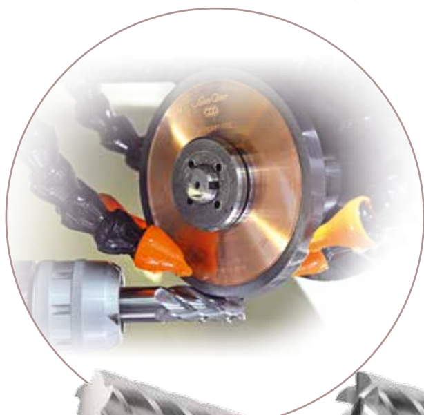
HYPERFLUTE+ Grinding tools 1A1
