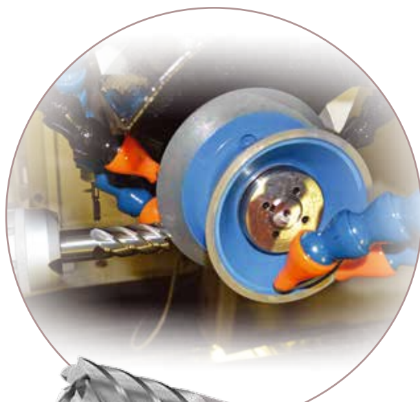
HYPER-G Grinding tools 11V9
